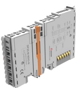
Digital input output module, 8 ports, NPN, 24VDC
