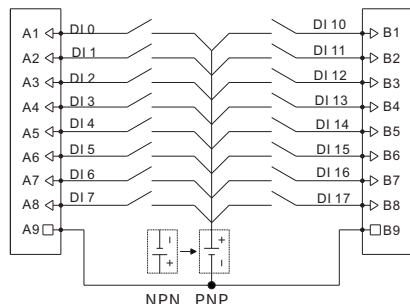
Wiring Diagram
