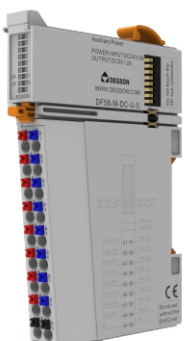
System power supply module, 24VDC to 5VDC
