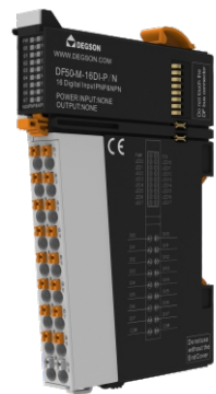
Digital input module, 16 ports, PNP, 24VDC
