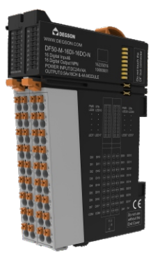
Digital input output module, 16-channel input+16-channel output, NPN, 24VDC
