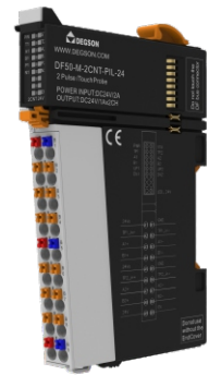
24V Pulse counting module,2 channel
