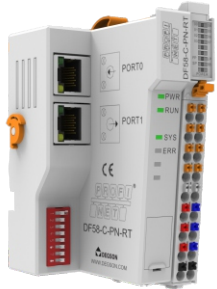
PROFINET, 2 RJ45, extensible 32 modules, 24VDC
