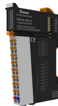
Digital output module, 16 ports, NPN, 24VDC
