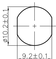
Panel cut
